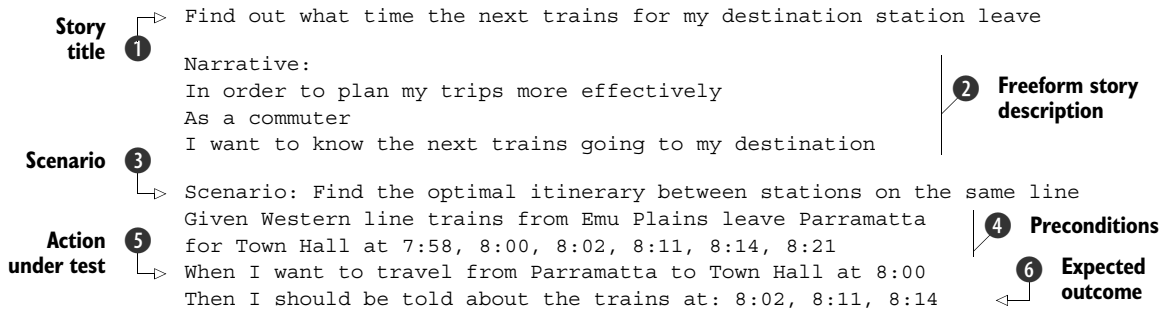
Listing 2.1 Acceptance criteria expressed in JBehave
